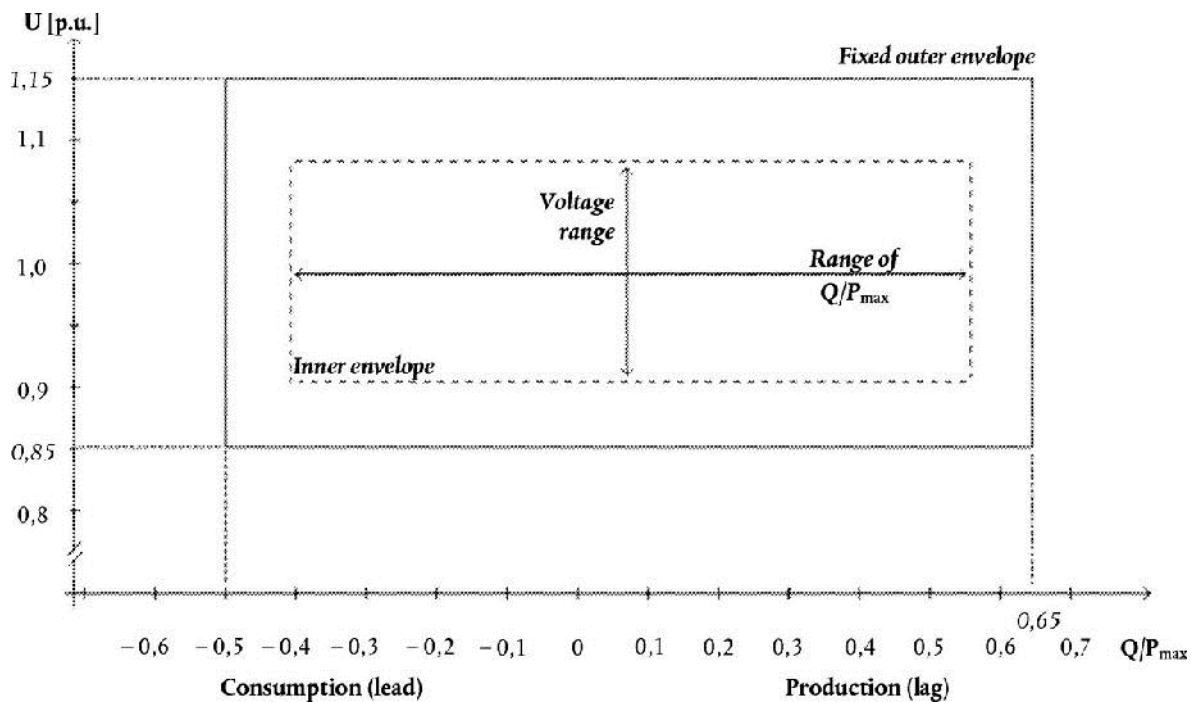
Figure 7: U-Q/P max -profile of a DC-connected power park module at the connection point. The diagram represents boundaries of a U-Q/P max -profile of the voltage at the connection point[s], expressed by the ratio of its actual value to its reference 1 pu value in per unit, against the ratio of the reactive power (Q) to the maximum capacity (P max ). The position, size and shape of the inner envelope are indicative and other than rectangular may be used within the inner envelope. For profile shapes other than rectangular, the voltage range represents the highest and lowest voltage points. Such a profile would not give rise to the full reactive power range being available across the range of steady-state voltages.
