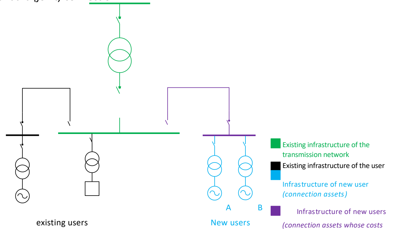
Standard (joint) connection
