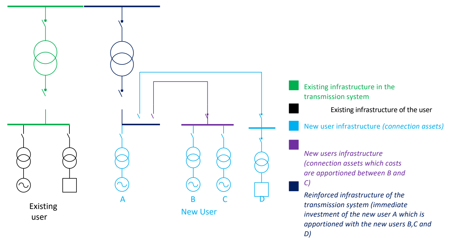
Reinforced Connection (joint one)
