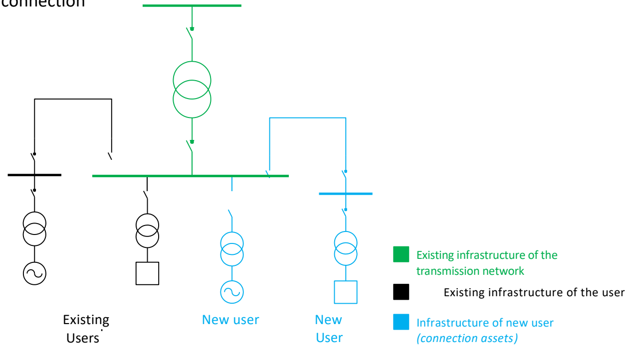
Standard connection
