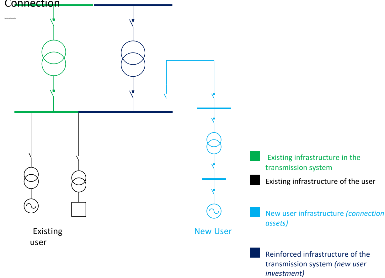
Reinforced Connection
